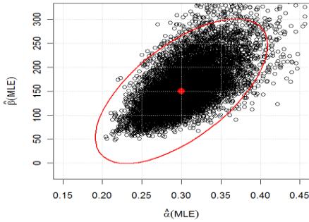
Figure 3: A 98% confidence ellipse for \alpha and \beta based on maximum likelihood estimates when \alpha = 0.3, \beta = 150 .
