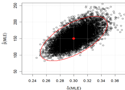
Figure 7: A 98% confidence ellipse for \alpha and \beta based on maximum likelihood estimates when \alpha = 0.3, \beta = 150 .
