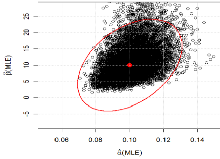
Figure 1: A 98% confidence ellipse for \alpha and \beta based on maximum likelihood estimates when \alpha = 0.1, \beta = 10 .
